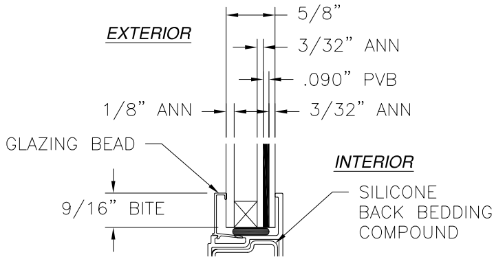
GLAZING DETAIL
